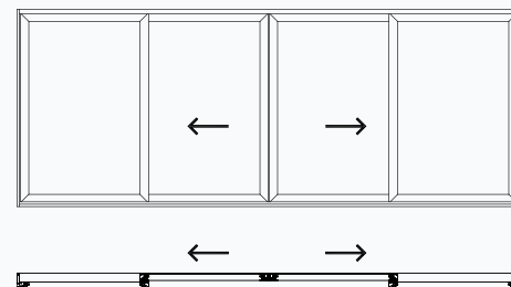
Four pane Single track lift and slide OXXO / OXXOH
